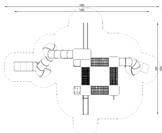
Top view with impact area
