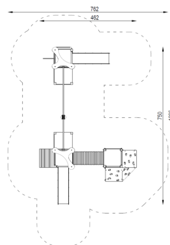
Top view with falling area
