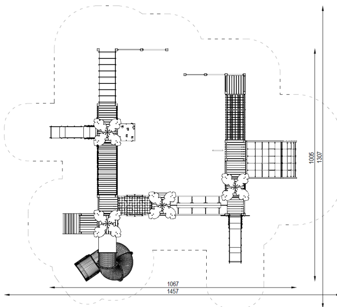
Top view with falling area
