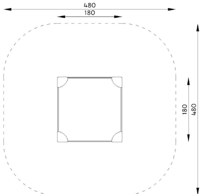
Top view with falling area
